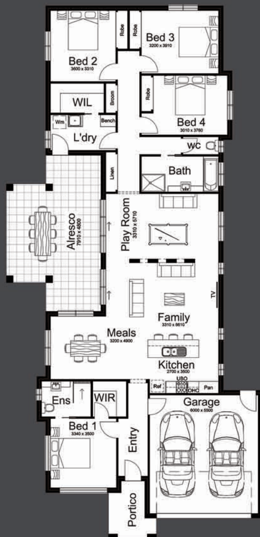
FLINDERS 19.7
